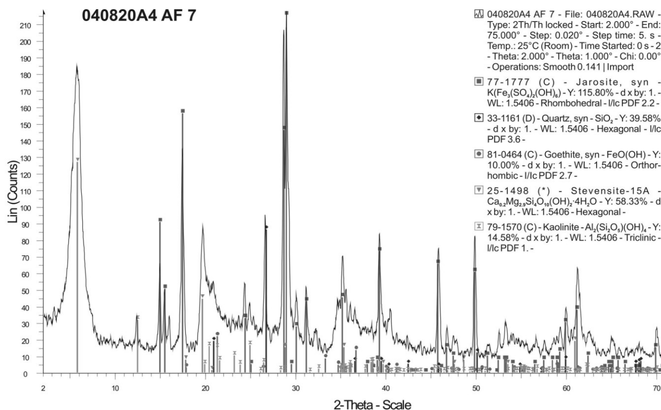
FIGURE 1 □: X-ray powder diffraction diagram of sample AF7.
