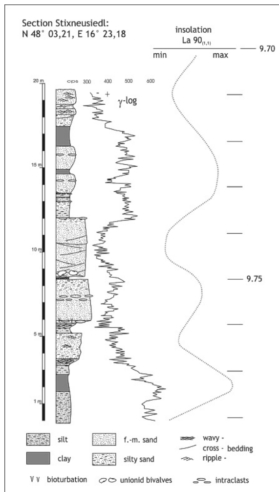
FIGURE 7: Based on the datings of the mammal faunas from Götzendorf and Stixneusiedl, the age of the Stixneusiedl section can roughly be estimated to range between 9.7 and 9.8 Ma. Although a straightforward correlation is impossible at present, a parallel trend of the \gamma -log pattern and the insolation curve could be alleged. The lower and upper maxima are well reflected by floodings and the deposition of clay, whilst the low-amplitude insolation maximum in the middle might relate to a weak flooding within a generally fluvial-influenced unit. However, autocyclic and/or tectonic overprint cannot be excluded.
