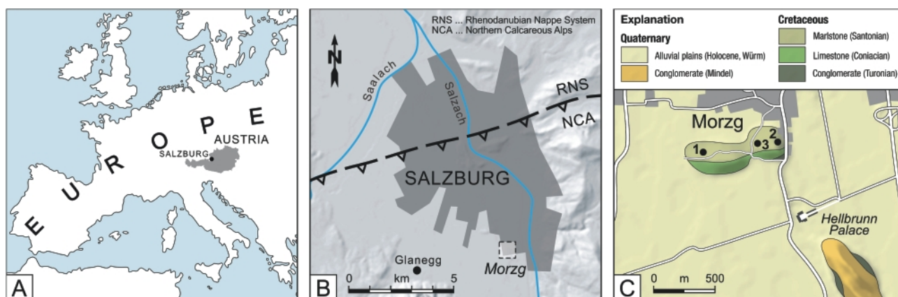
FIGURE 1: A,B...Geographical maps showing the position of the studied area, C....Geological sketch map of the Morzg area modified after Prey (1969) and position of the sampled outcrops (1...Morzg West, 2...Morzg Ost, 3...Rö).
