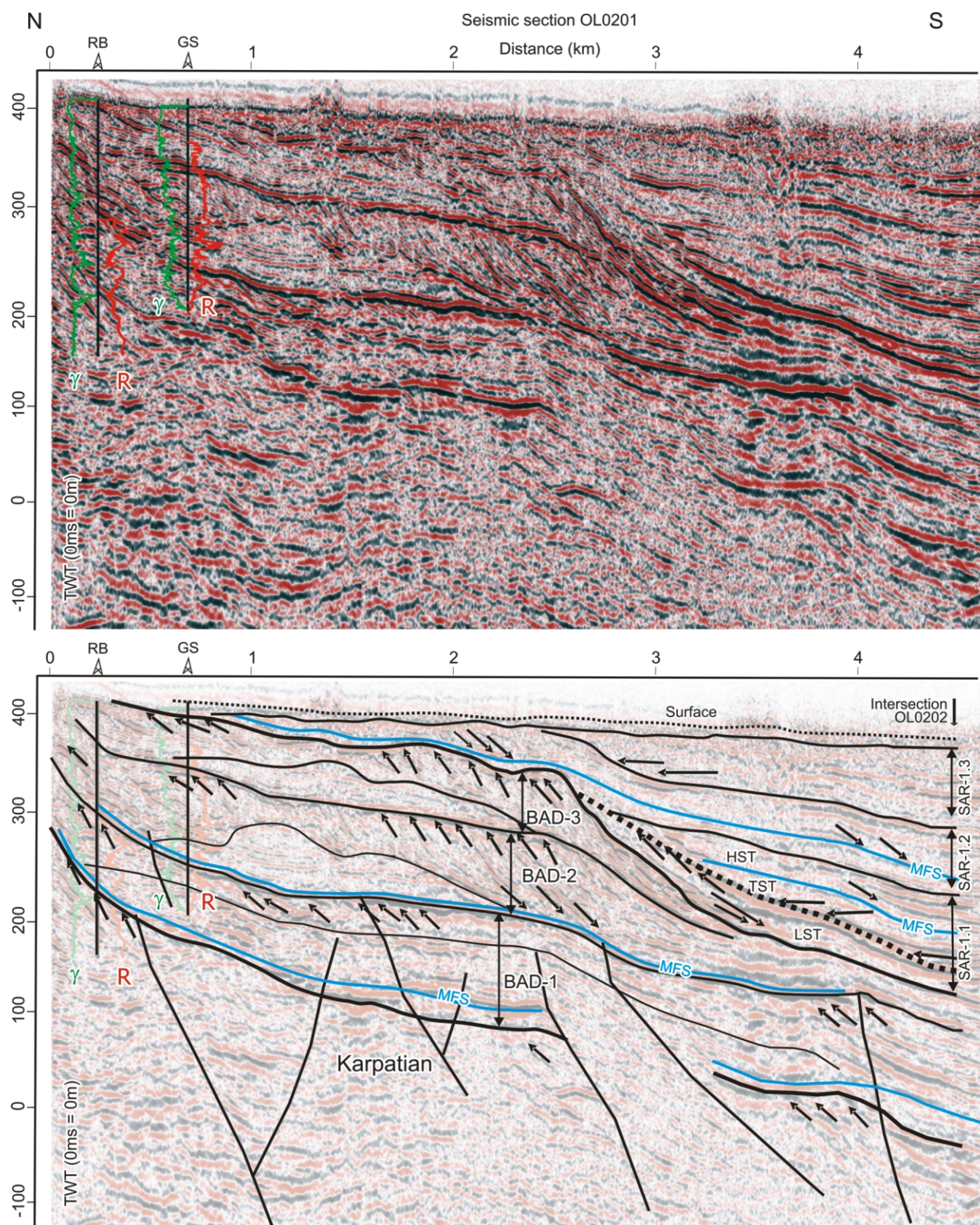
FIGURE 4: N-S seismic section OL0201 with gamma (γ) and resistivity (R) logs of wells RB and GS. See Figure 1 for location of seismic section.
