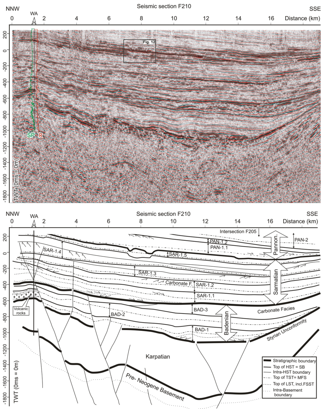
FIGURE 7: Seismic section F210 with Spontaneous Potential (SP) and resistivity (R) logs of well Walkersdorf 1 (WA) and its interpretation. See Figure 1 for position of seismic section.
