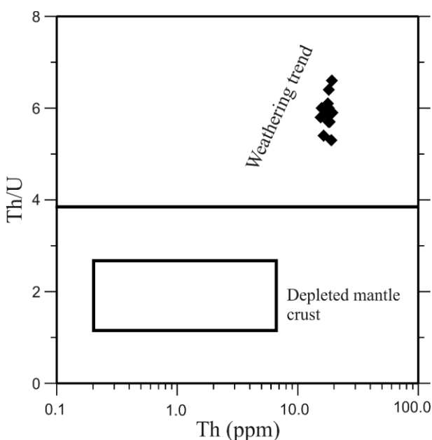
FIGURE 9: Plots of \text{Th}/\text{U} versus \text{Th} (after McLennan et al., 1993).
