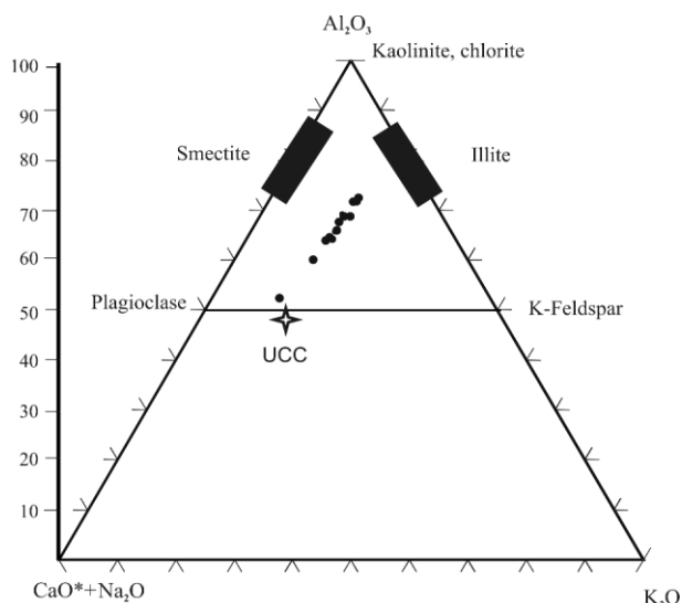
FIGURE 8: CIA ternary diagram, \text{Al}_2\text{O}_3 - \text{CaO}^* - \text{Na}_2\text{O} - \text{K}_2\text{O} (after Nesbit and Young, 1982); \text{CaO}^* = \text{CaO} in silicate phase.
